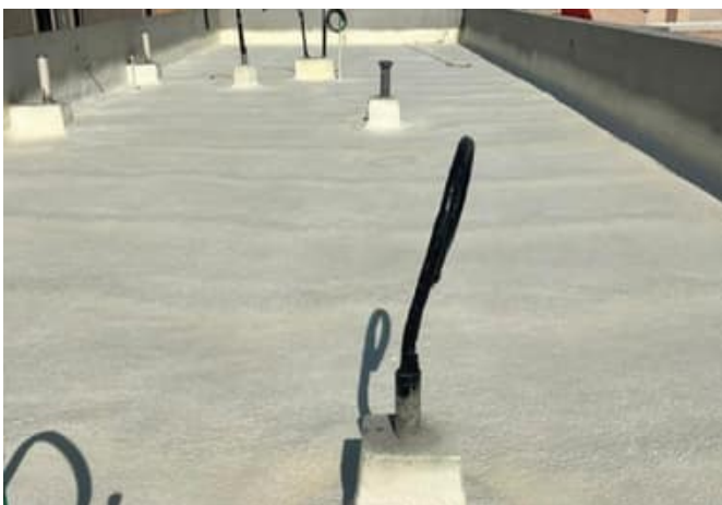
Roof waterproofing
