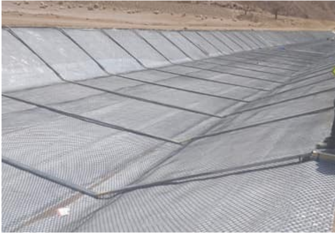
Channel on a slope
